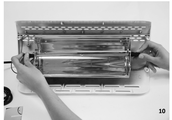
10. REASSEMBLE THE DEVICE BY PERFORMING THE ABOVE TASKS IN REVERSE ORDER.
