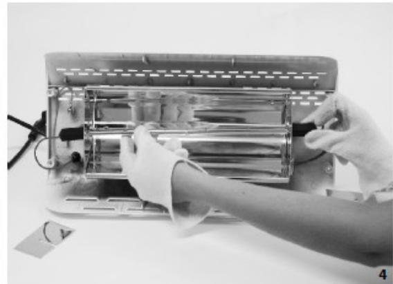
4. EXTRACT THE BULB FROM THE SPRING CLIPS.
